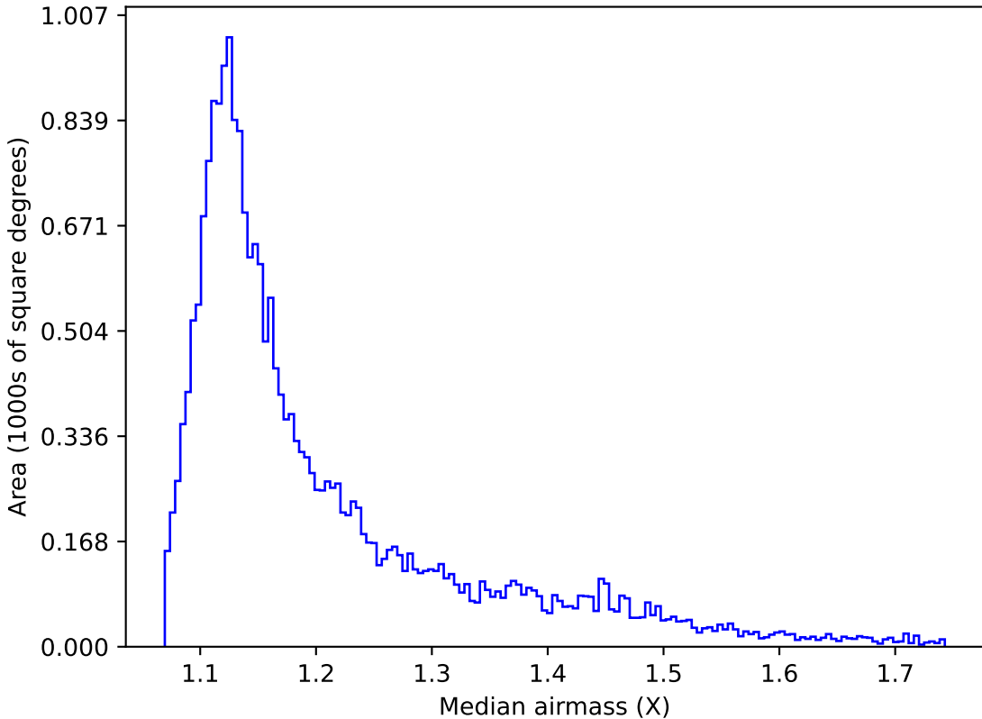
early_u_fpextra3.0_v3.4_10yrs Yr 1 y band: Median airmass
