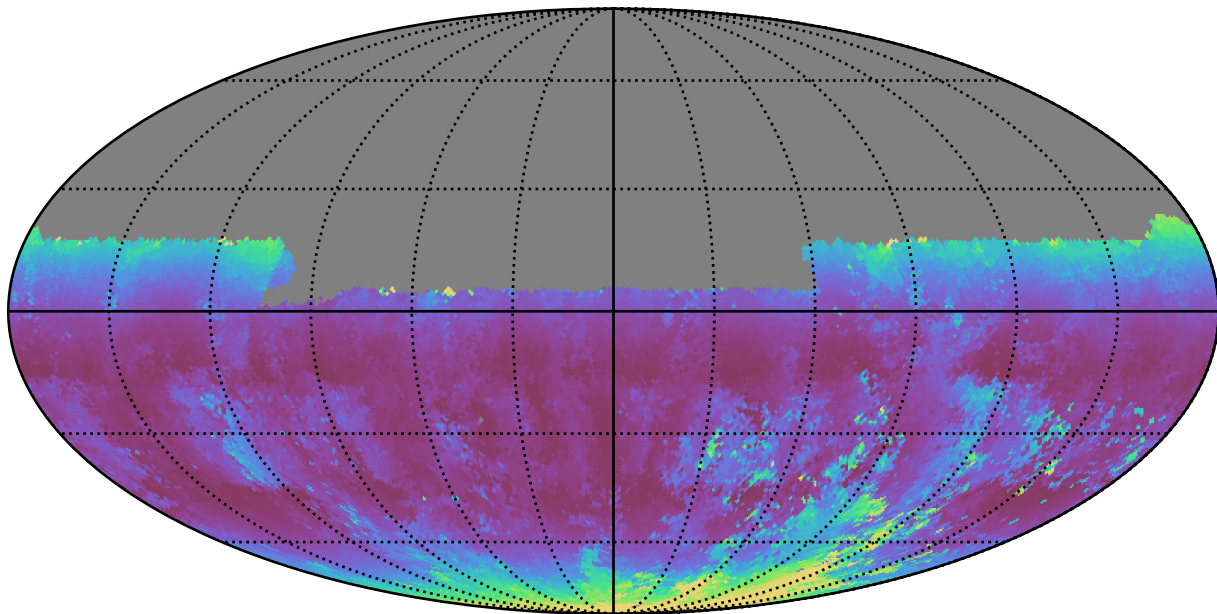
early_u_fpextra3.0_v3.4_10yrs Yr 1 u band: Median airmass
