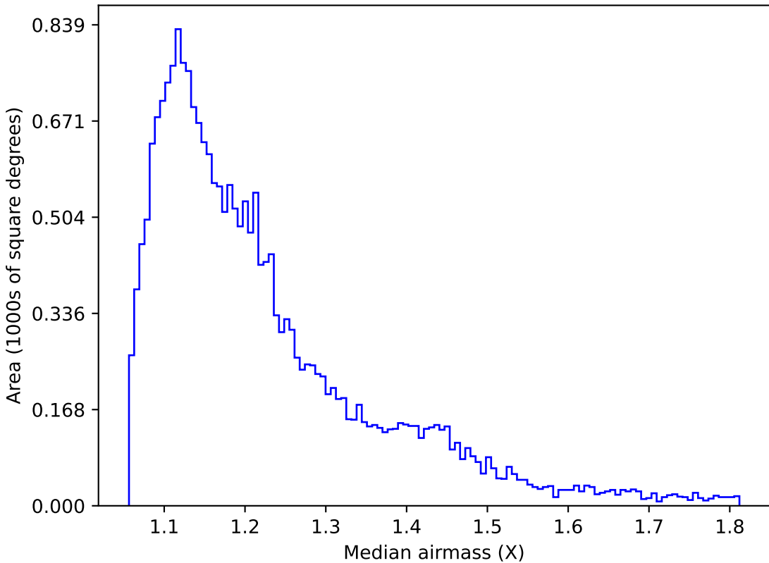
early_u_fpextra3.0_v3.4_10yrs Yr 1 u band: Median airmass
