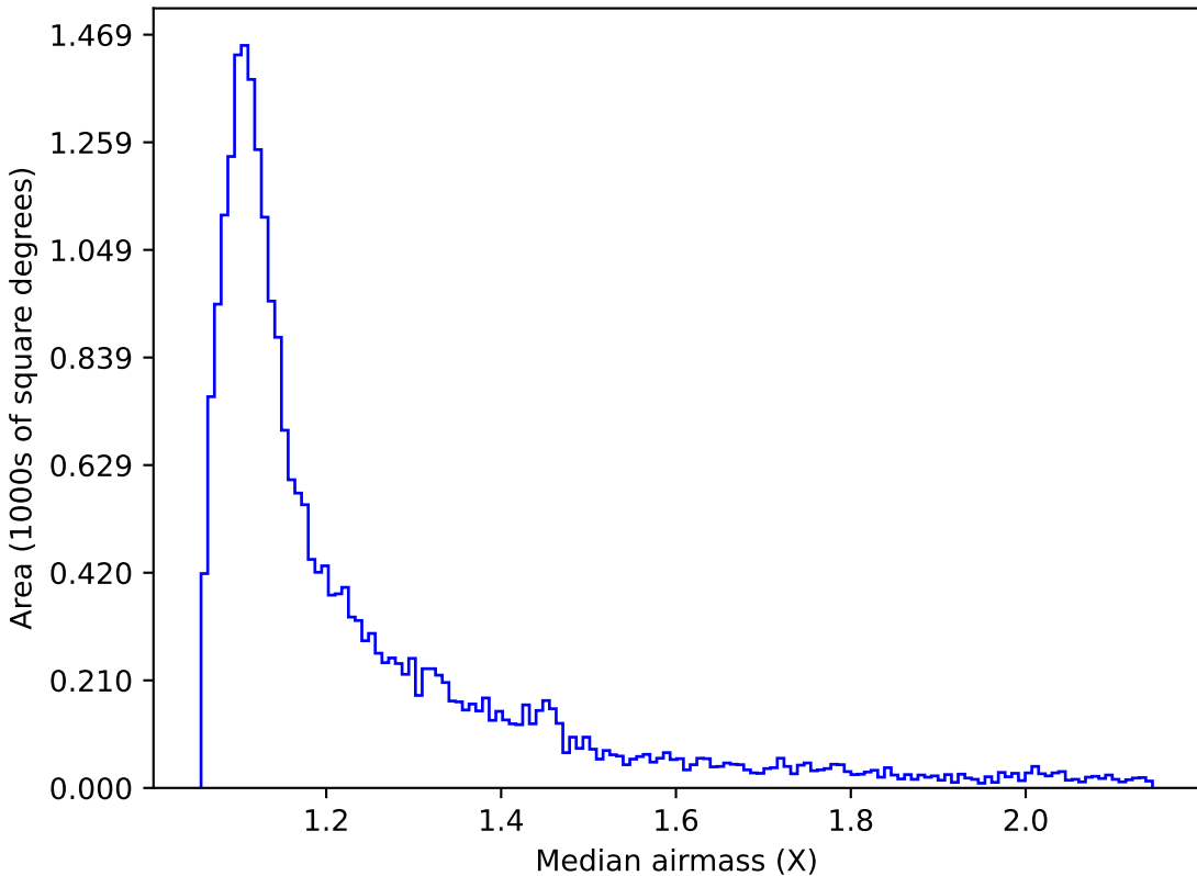
early_u_fpextra3.0_v3.4_10yrs Yr 1 r band: Median airmass
