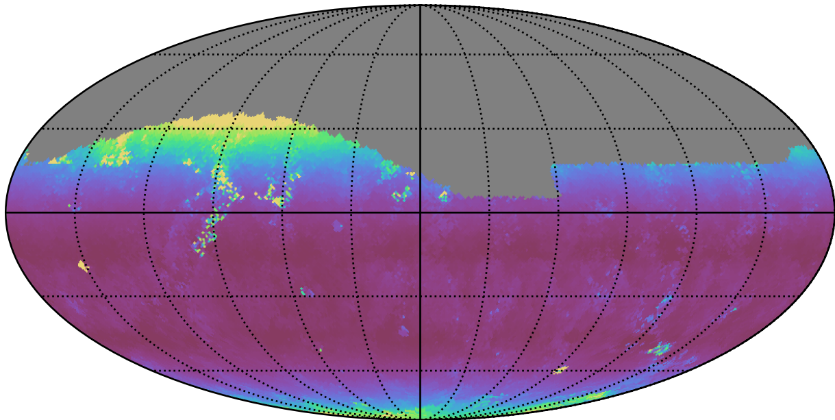
early_u_fpextra3.0_v3.4_10yrs Yr 1 i band: Median airmass
