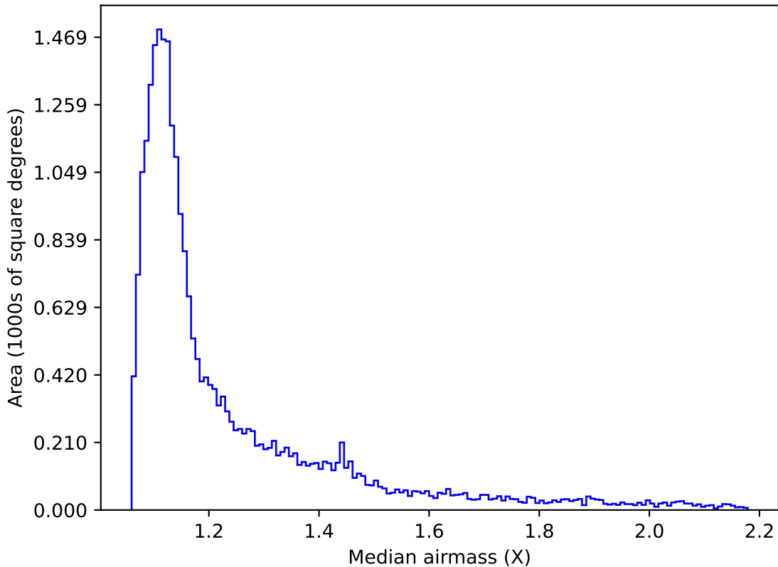
early_u_fpextra3.0_v3.4_10yrs Yr 1 i band: Median airmass
