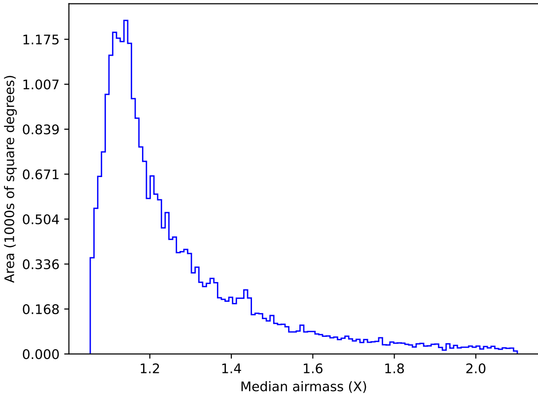
early_u_fpextra3.0_v3.4_10yrs Yr 1 g band: Median airmass
