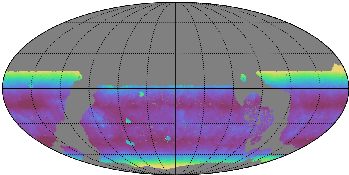
early_u_fpextra3.0_v3.4_10yrs WFD z band: Median airmass
