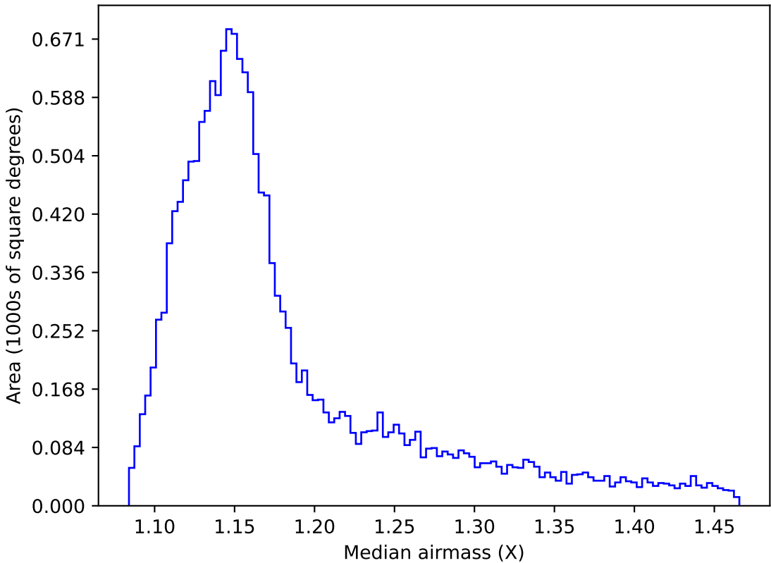
early_u_fpextra3.0_v3.4_10yrs WFD z band: Median airmass
