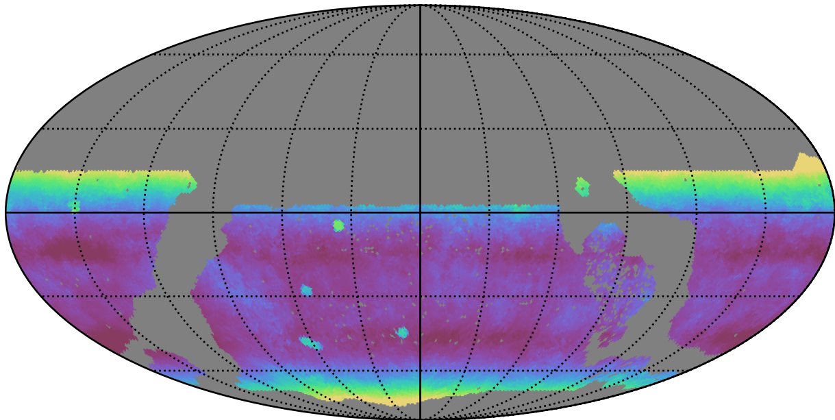
early_u_fpextra3.0_v3.4_10yrs WFD y band: Median airmass
