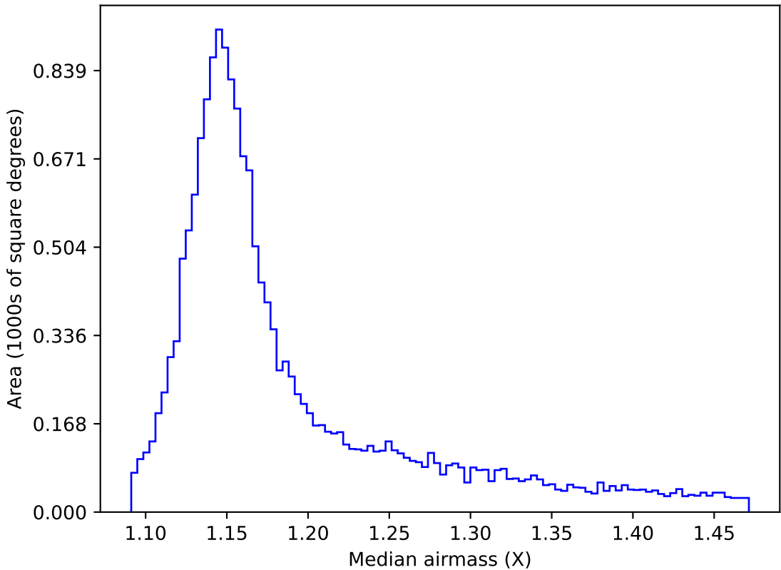
early_u_fpextra3.0_v3.4_10yrs WFD y band: Median airmass
