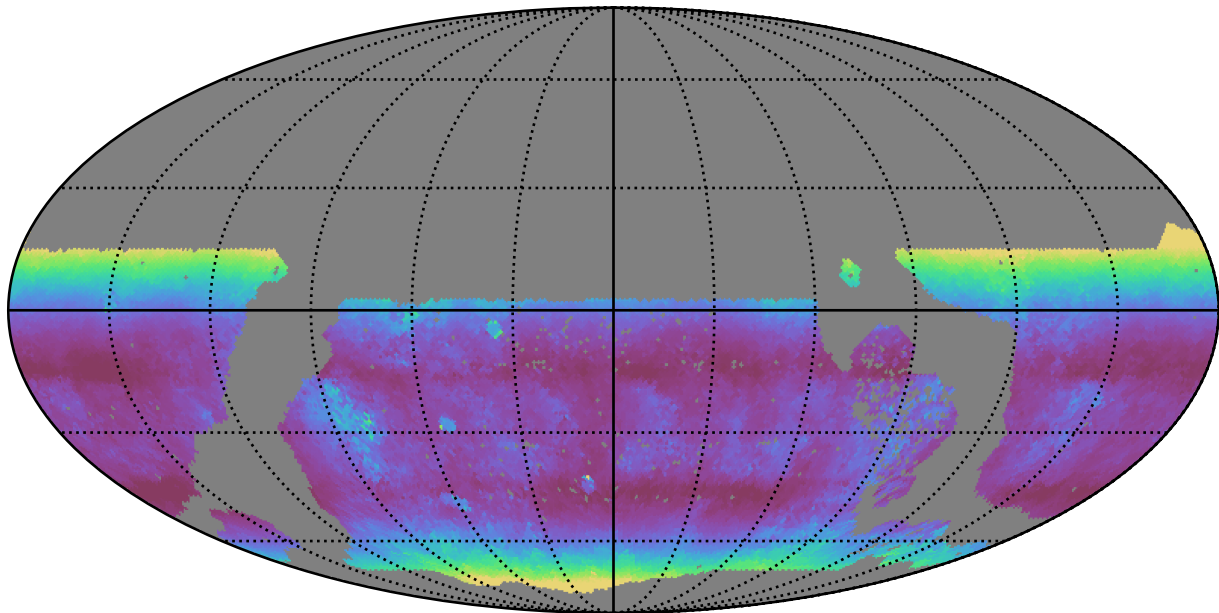
early_u_fpextra3.0_v3.4_10yrs WFD u band: Median airmass
