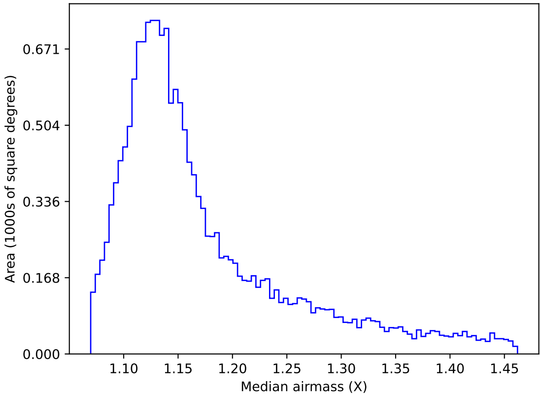
early_u_fpextra3.0_v3.4_10yrs WFD u band: Median airmass
