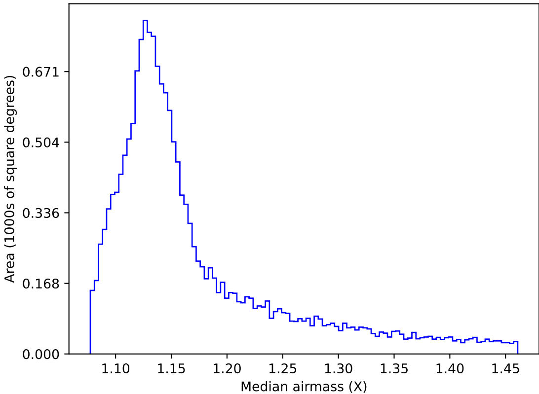
early_u_fpextra3.0_v3.4_10yrs WFD r band: Median airmass
