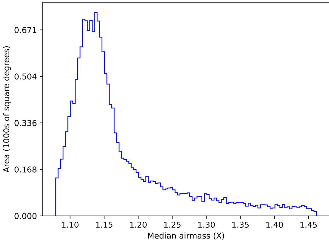
early_u_fpextra3.0_v3.4_10yrs WFD i band: Median airmass
