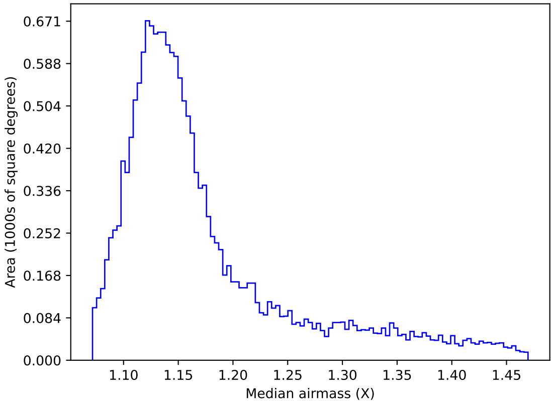
early_u_fpextra3.0_v3.4_10yrs WFD g band: Median airmass
