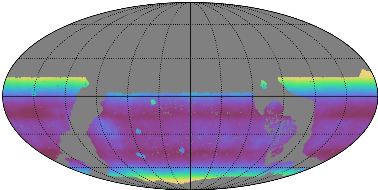
early_u_fpextra3.0_v3.4_10yrs WFD all bands: Median airmass
