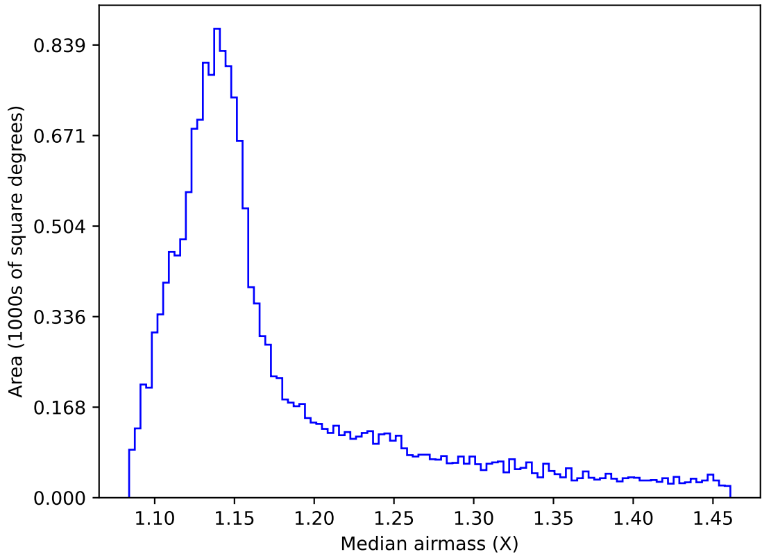
early_u_fpextra3.0_v3.4_10yrs WFD all bands: Median airmass
