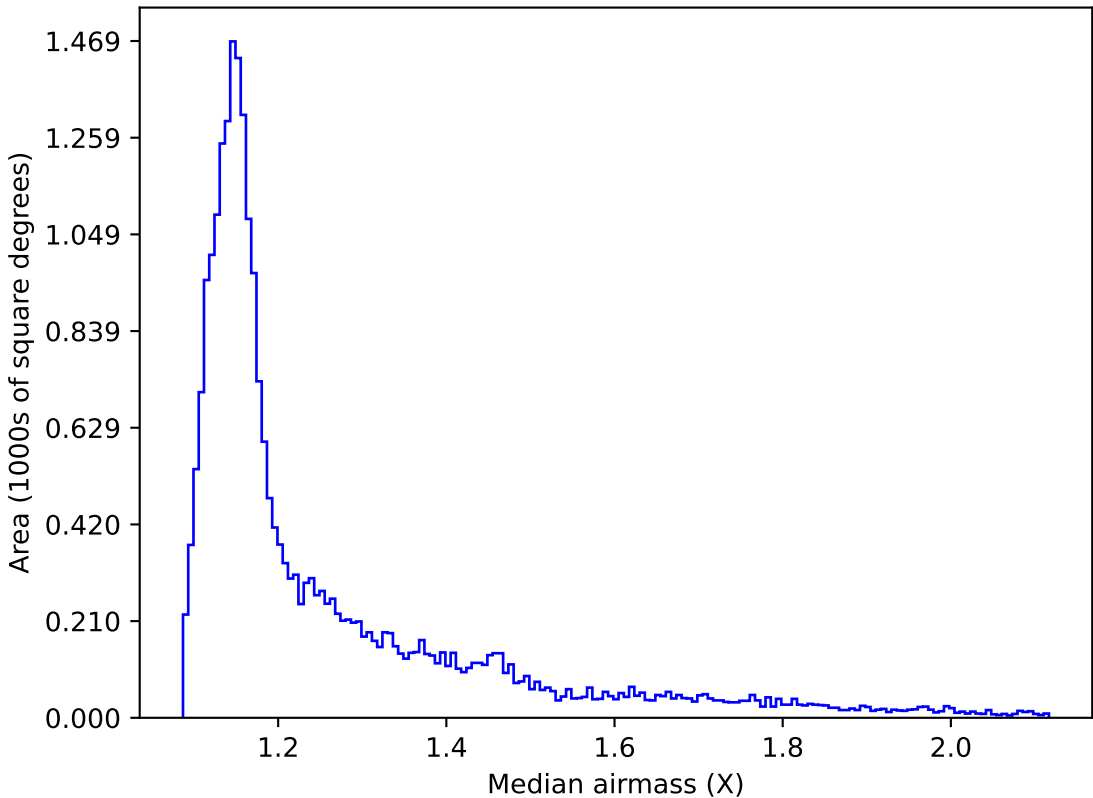
early_u_fpextra3.0_v3.4_10yrs All sky z band: Median airmass
