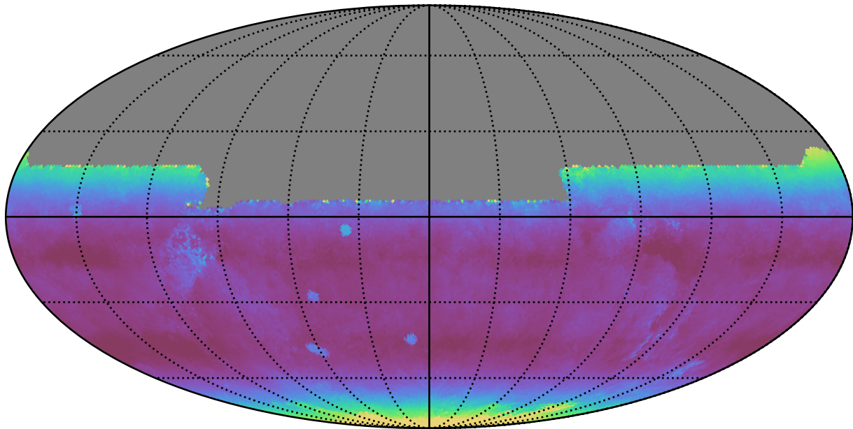
early_u_fpextra3.0_v3.4_10yrs All sky y band: Median airmass
