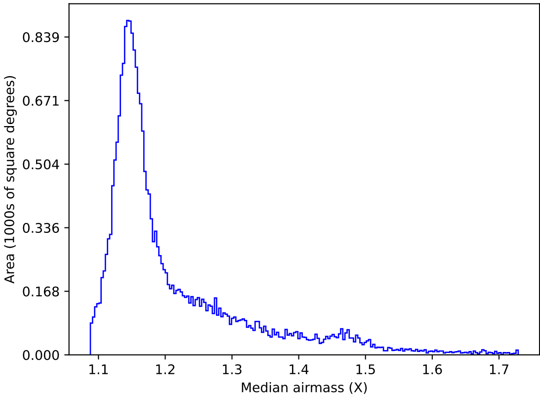
early_u_fpextra3.0_v3.4_10yrs All sky y band: Median airmass
