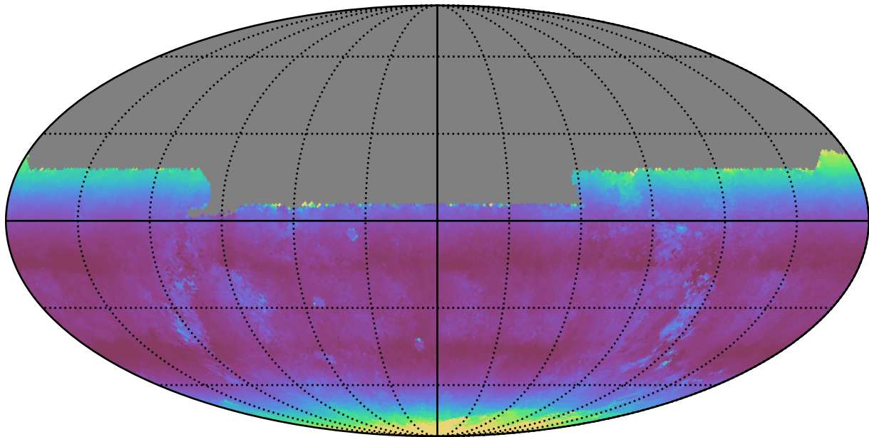
early_u_fpextra3.0_v3.4_10yrs All sky u band: Median airmass
