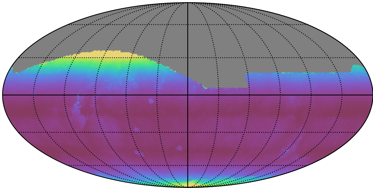
early_u_fpextra3.0_v3.4_10yrs All sky r band: Median airmass
