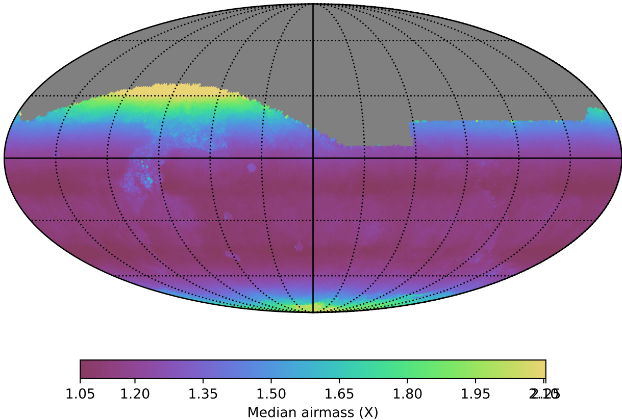
early_u_fpextra3.0_v3.4_10yrs All sky i band: Median airmass
