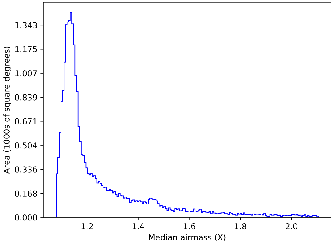
early_u_fpextra3.0_v3.4_10yrs All sky i band: Median airmass
