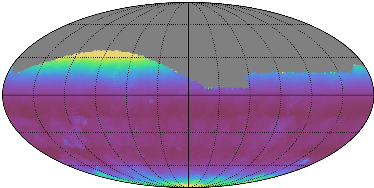
early_u_fpextra3.0_v3.4_10yrs All sky g band: Median airmass
