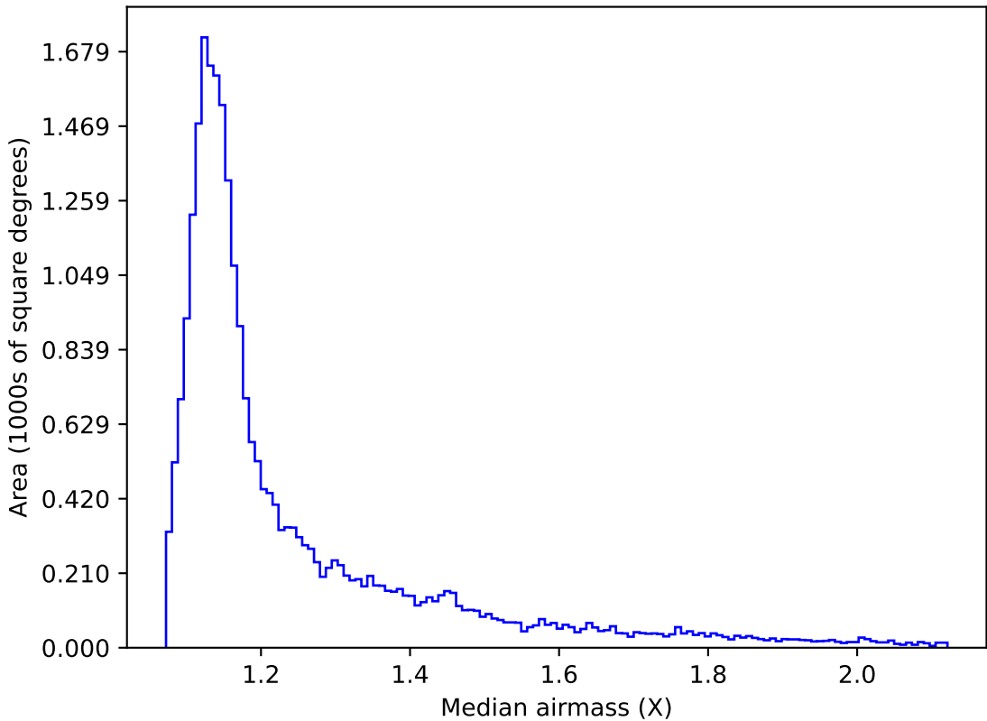
early_u_fpextra3.0_v3.4_10yrs All sky g band: Median airmass
