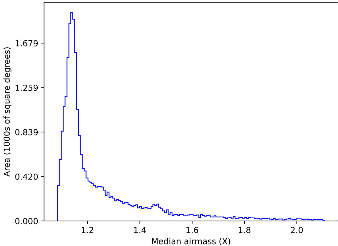
early_u_fpextra3.0_v3.4_10yrs All sky all bands: Median airmass
