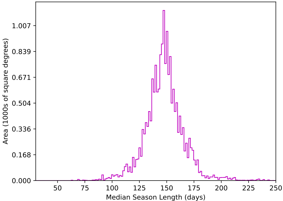
early_u_fpextra3.0_v3.4_10yrs WFD z band: Median Season Length
