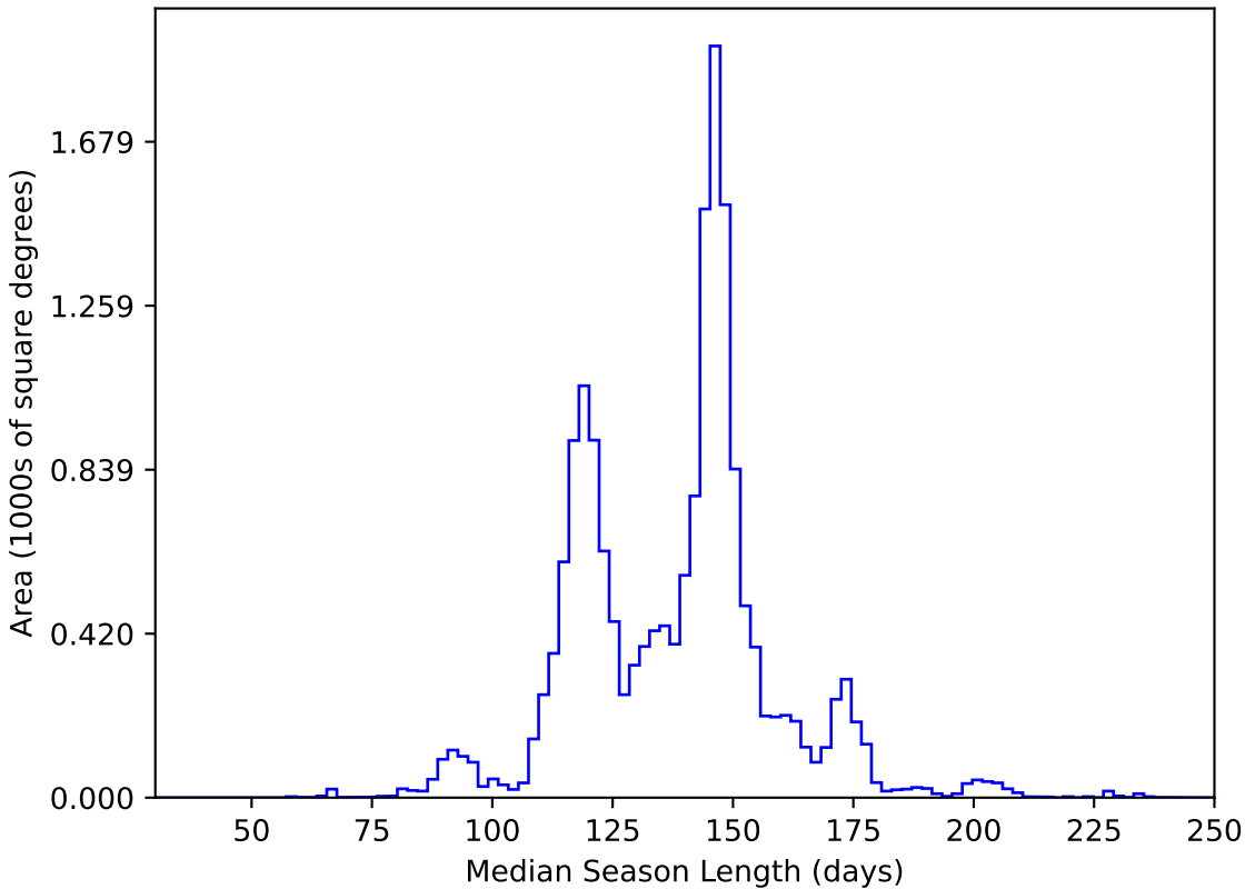
early_u_fpextra3.0_v3.4_10yrs WFD y band: Median Season Length
