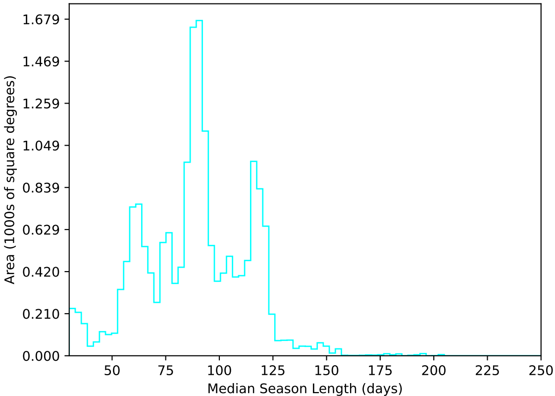
early_u_fpextra3.0_v3.4_10yrs WFD u band: Median Season Length
