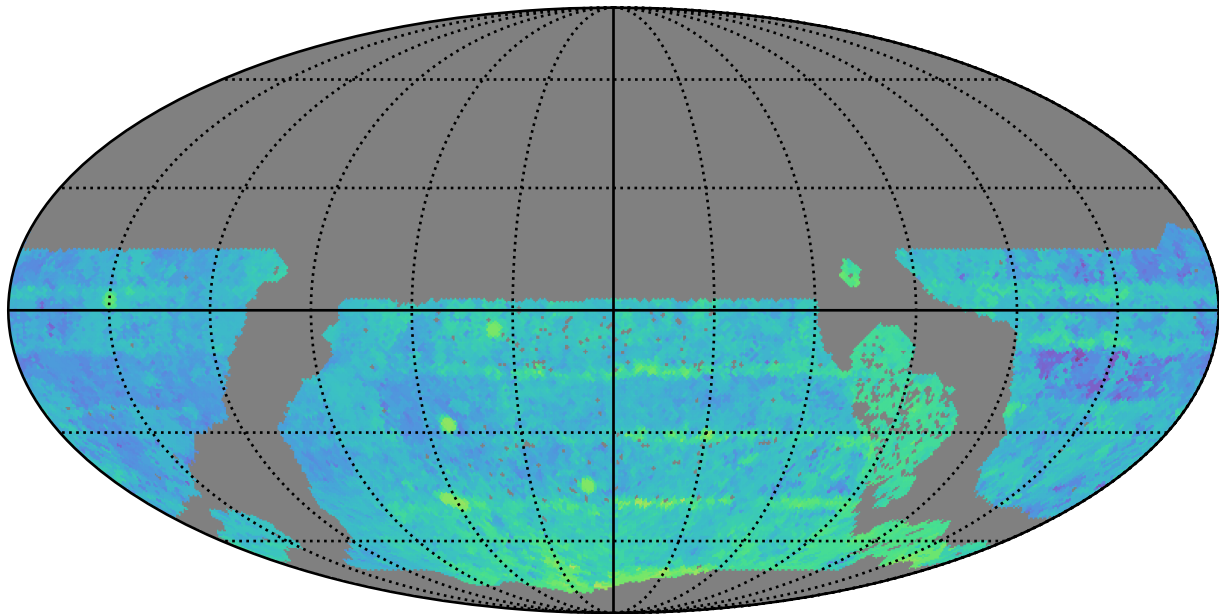
early_u_fpextra3.0_v3.4_10yrs WFD r band: Median Season Length
