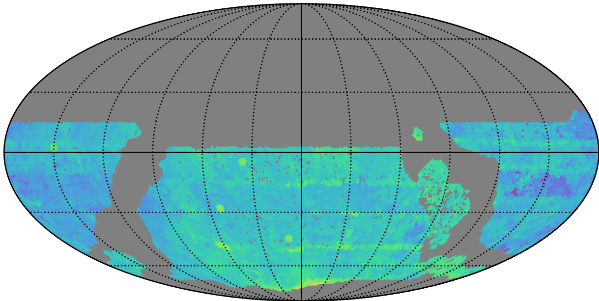
early_u_fpextra3.0_v3.4_10yrs WFD i band: Median Season Length
