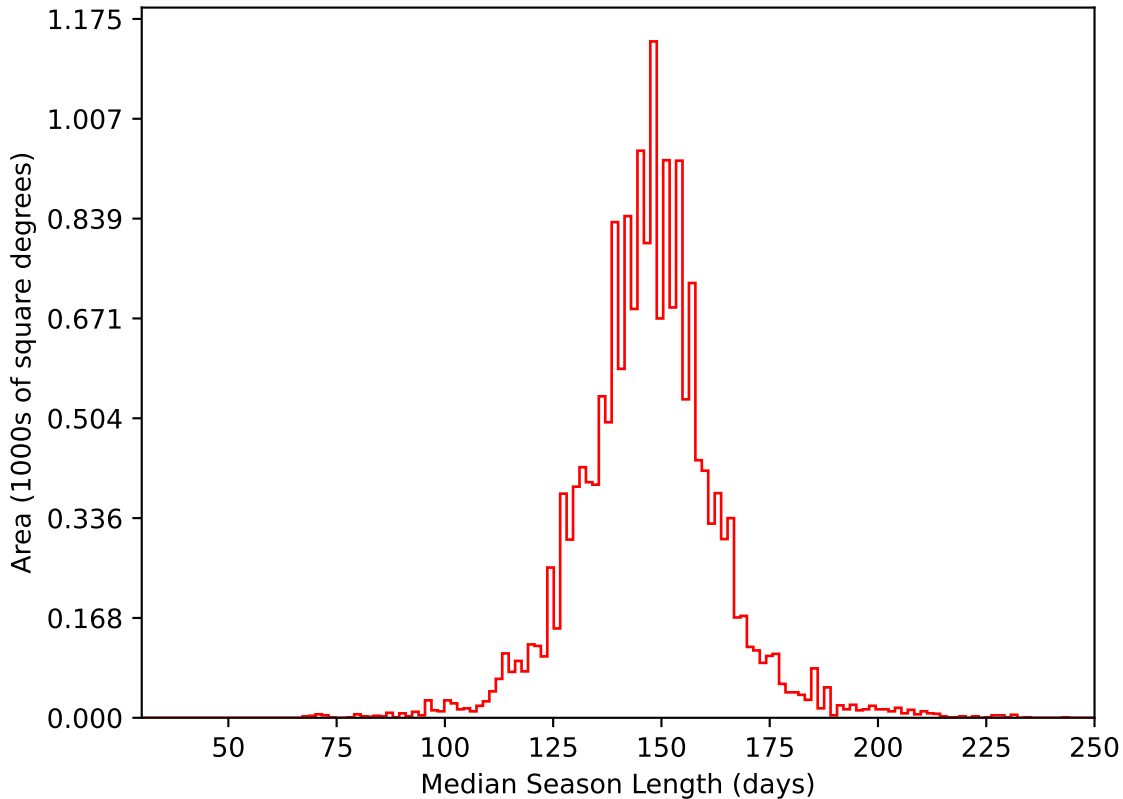
early_u_fpextra3.0_v3.4_10yrs WFD i band: Median Season Length
