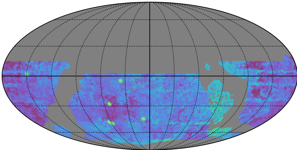
early_u_fpextra3.0_v3.4_10yrs WFD g band: Median Season Length
