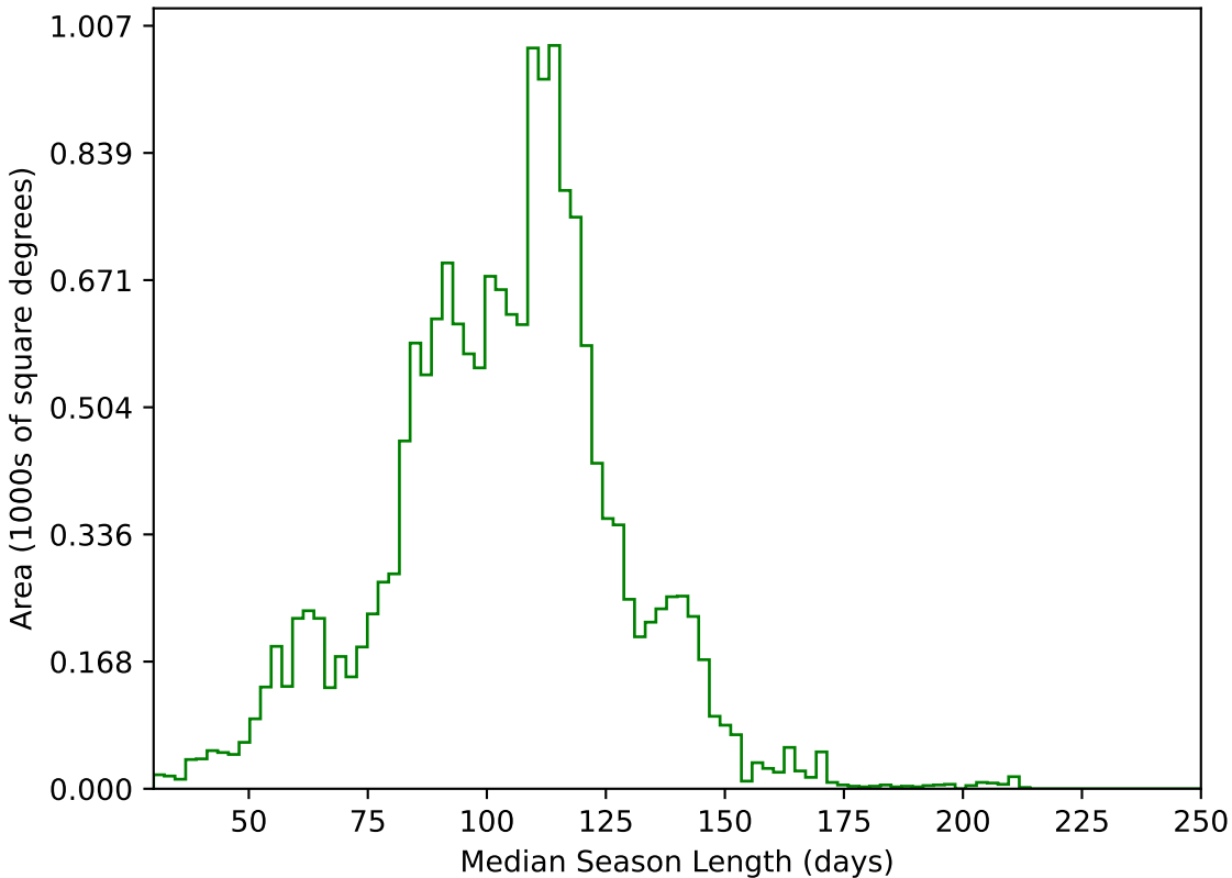
early_u_fpextra3.0_v3.4_10yrs WFD g band: Median Season Length
