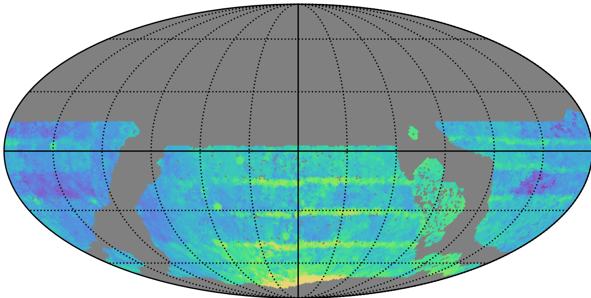
early_u_fpextra3.0_v3.4_10yrs WFD all bands: Median Season Length
