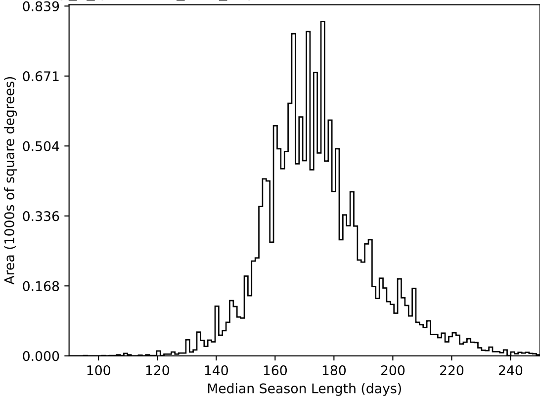
early_u_fpextra3.0_v3.4_10yrs WFD all bands: Median Season Length
