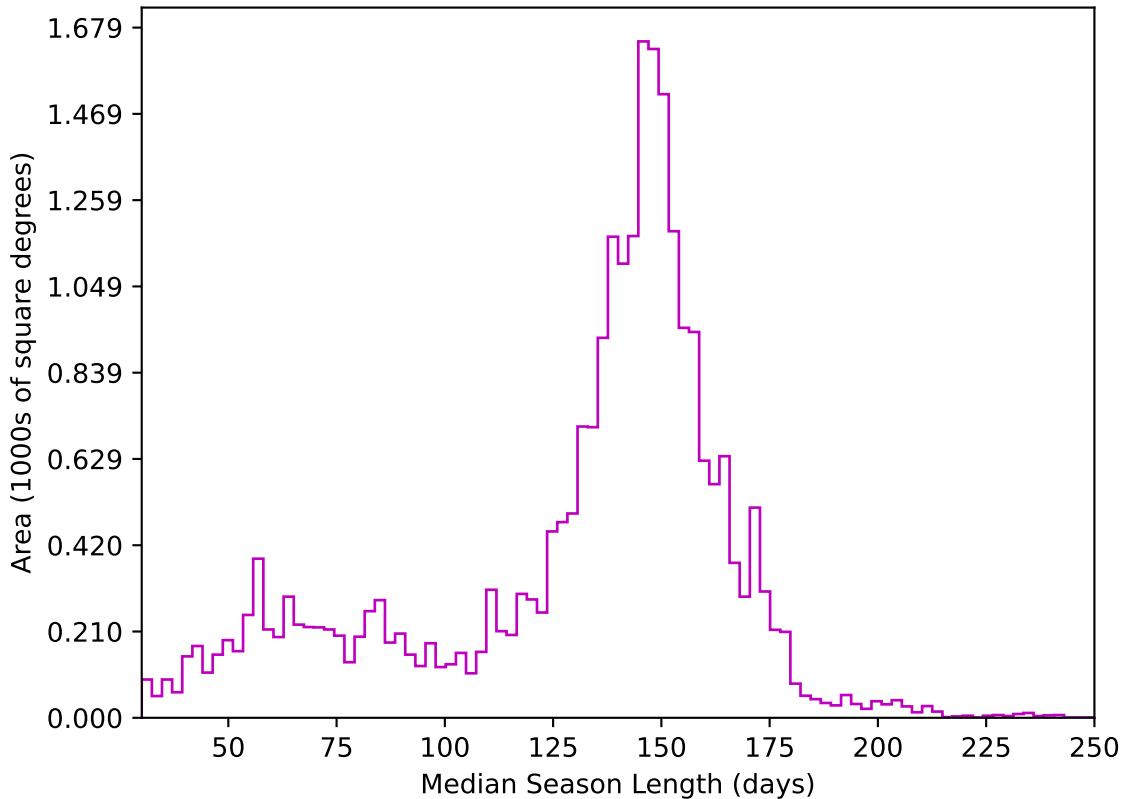
early_u_fpextra3.0_v3.4_10yrs All sky z band: Median Season Length
