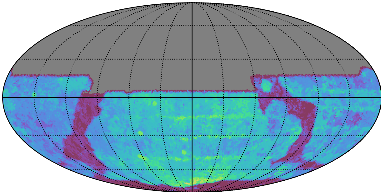
early_u_fpextra3.0_v3.4_10yrs All sky y band: Median Season Length
