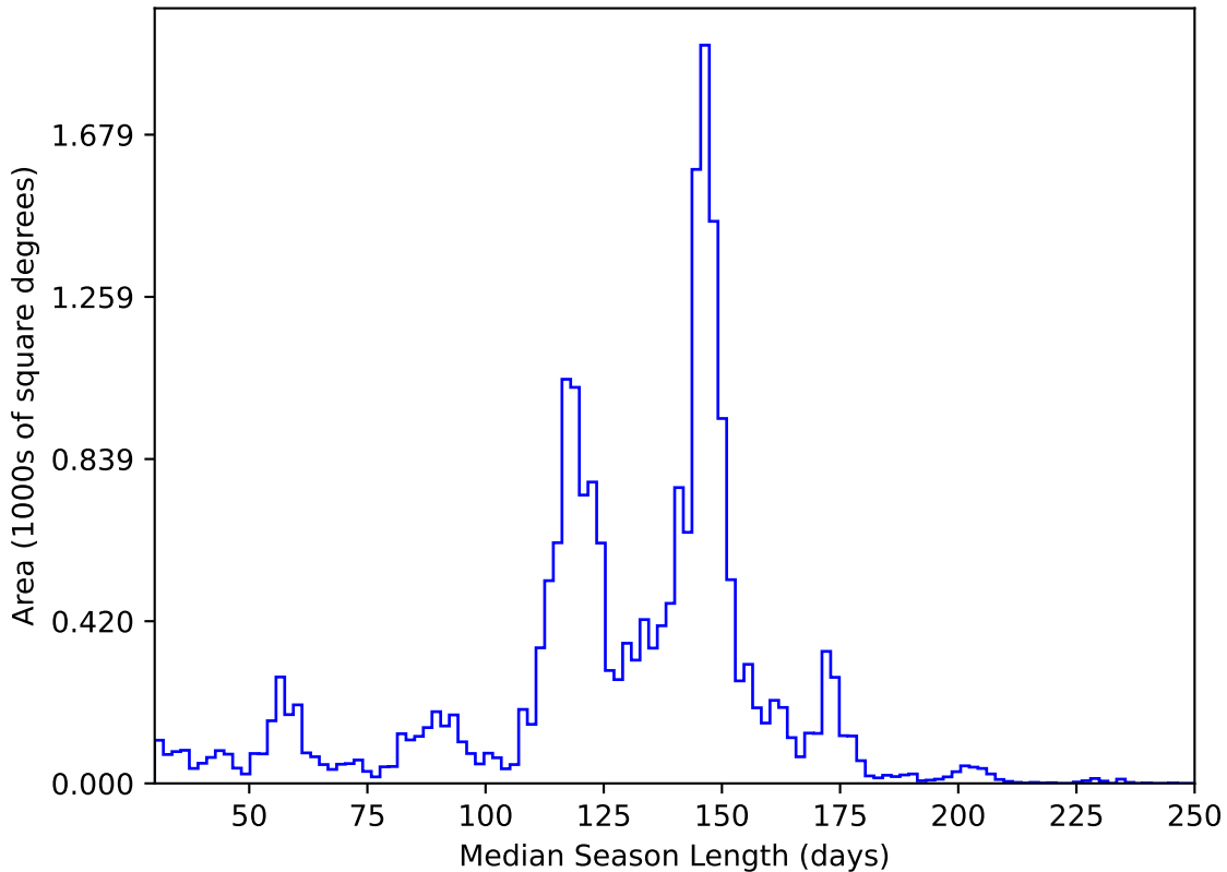
early_u_fpextra3.0_v3.4_10yrs All sky y band: Median Season Length
