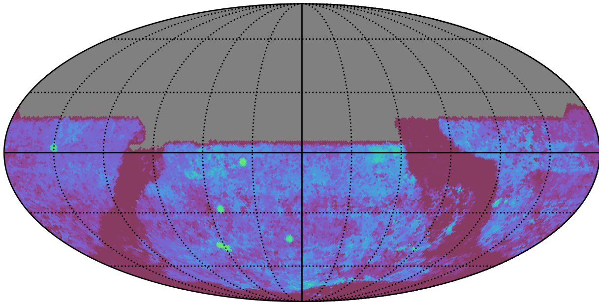
early_u_fpextra3.0_v3.4_10yrs All sky u band: Median Season Length
