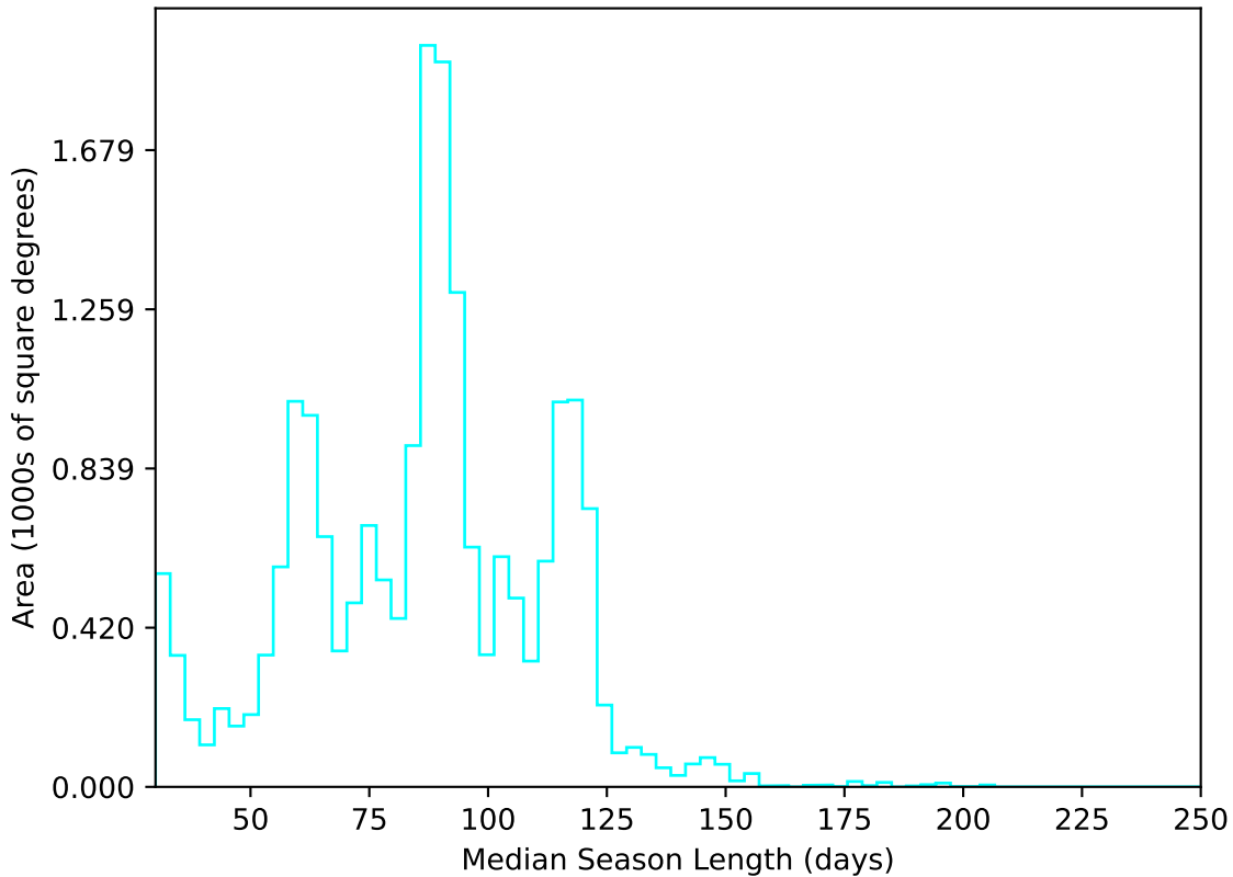
early_u_fpextra3.0_v3.4_10yrs All sky u band: Median Season Length
