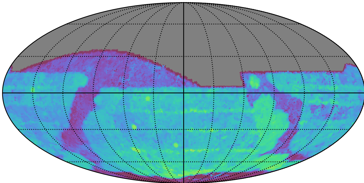
early_u_fpextra3.0_v3.4_10yrs All sky r band: Median Season Length
