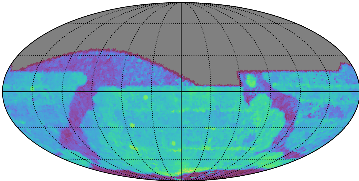
early_u_fpextra3.0_v3.4_10yrs All sky i band: Median Season Length
