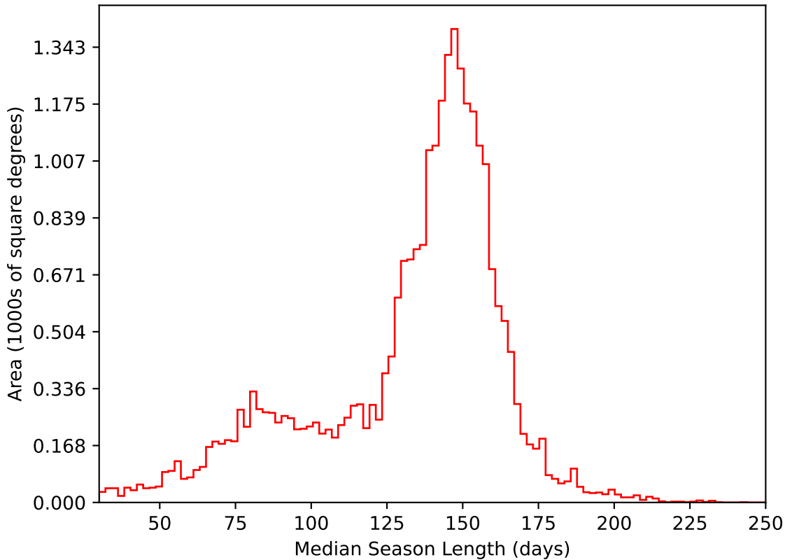
early_u_fpextra3.0_v3.4_10yrs All sky i band: Median Season Length
