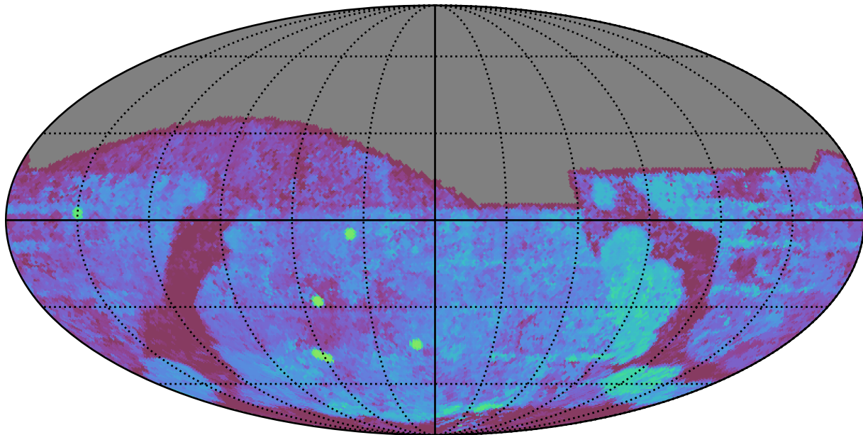
early_u_fpextra3.0_v3.4_10yrs All sky g band: Median Season Length
