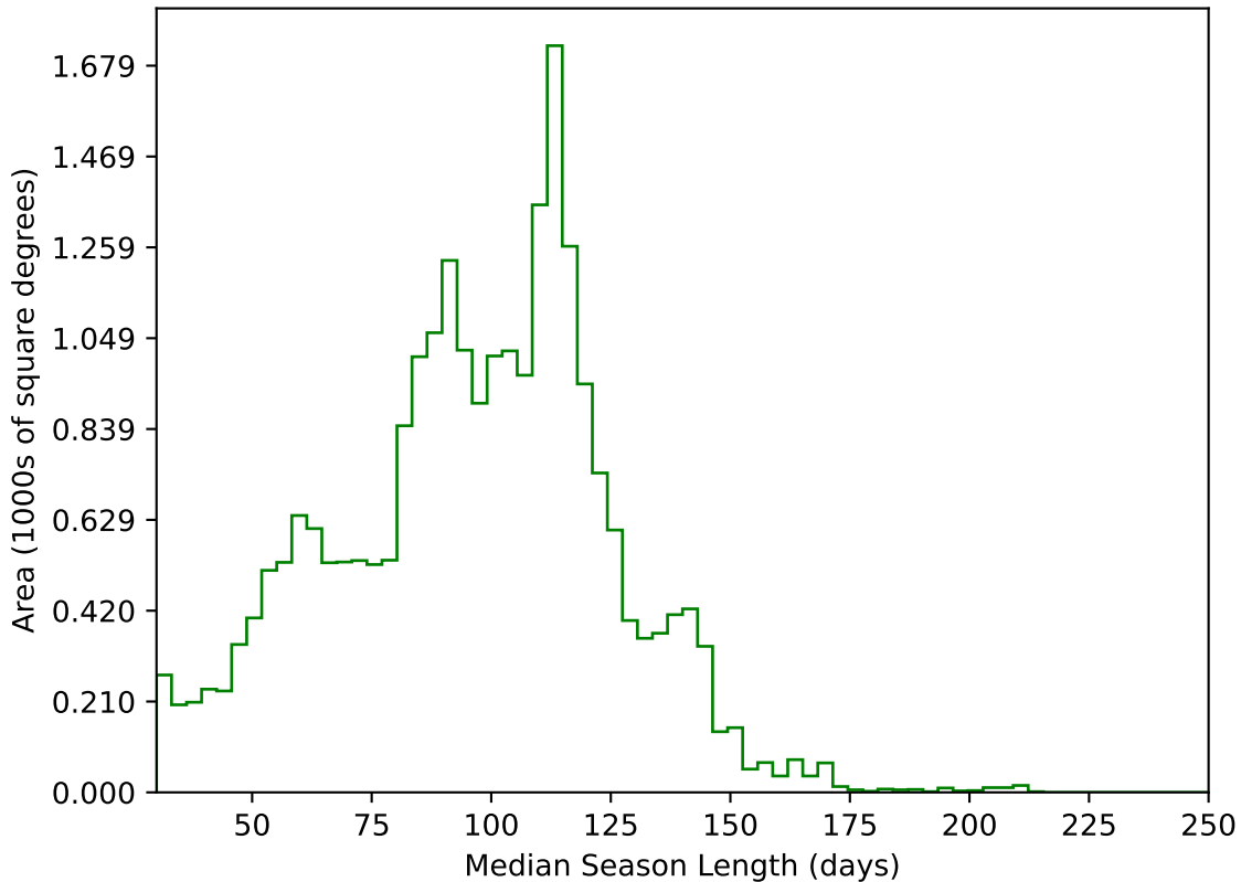
early_u_fpextra3.0_v3.4_10yrs All sky g band: Median Season Length
