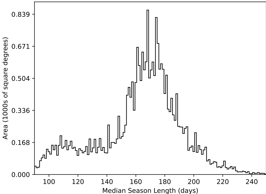
early_u_fpextra3.0_v3.4_10yrs All sky all bands: Median Season Length
