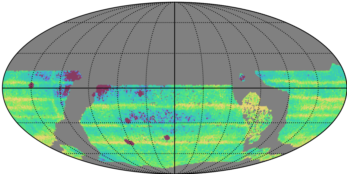
early_u_fpextra3.0_v3.4_10yrs WFD: Median Intra-Night Gap
